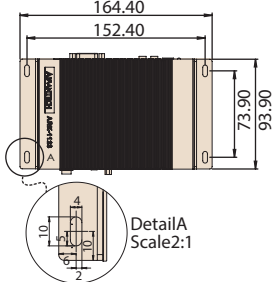
Wall mount
