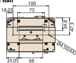
VESA mount
