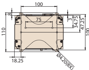
VESA mount
