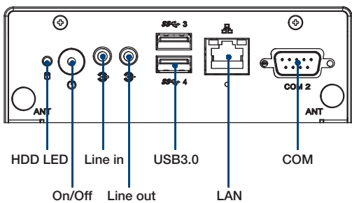
Front Panel External I/O Mechanical Layout/Drawing
