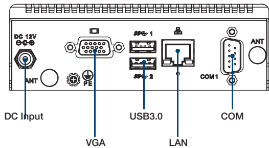
Rear Panel External I/O Mechanical Layout/Drawing
