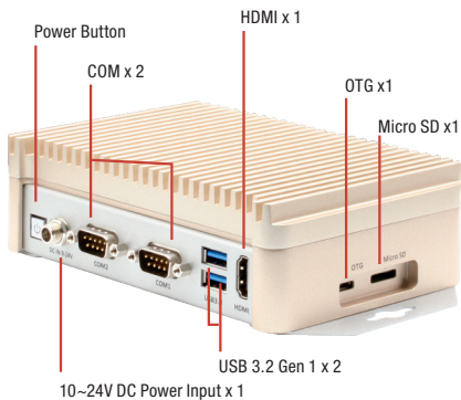
BOXER-8120AI-A1-CS-N0001 Front View
