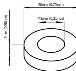
Terminal Dimensions
