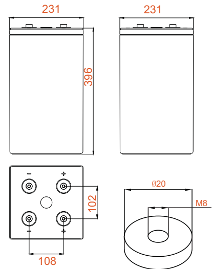
Terminal Dimensions
