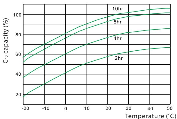
Capacity vs temperature curve
